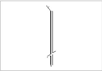
Ground spikes made from T-iron for a fixture with locking clips Length: 1250 mm with welded-on locking rail and cross rail at a height of 250 mm Order no.: GL 1500 920 125
